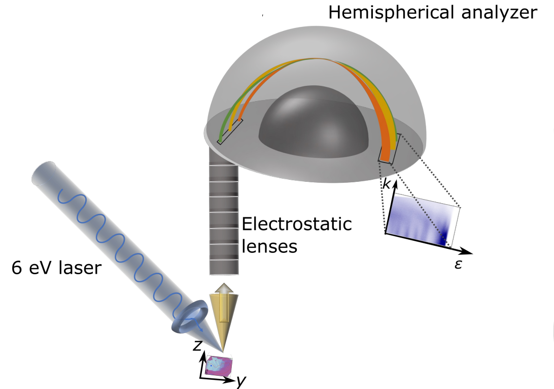
Photoemission Spectroscopy
